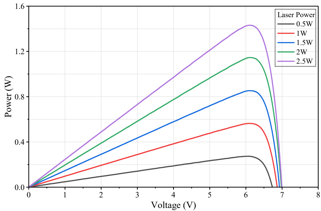
Figure 2: PV curve of MT020-808-600mW
