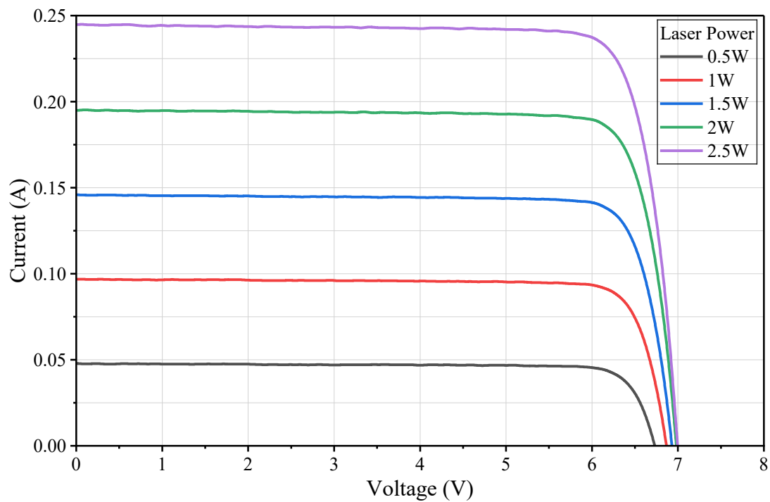
Figure 3: IV curve of MT020-808-600mW
